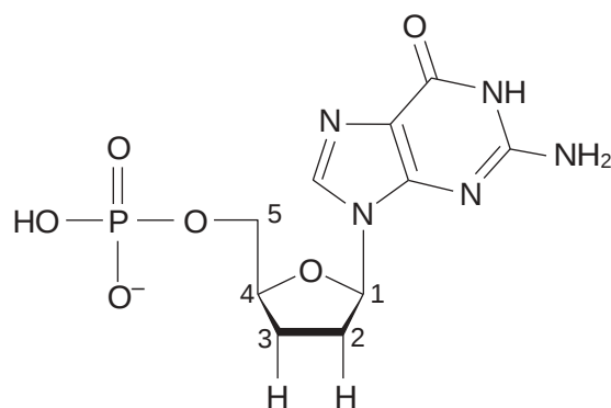
dideoxyribonucleotide
