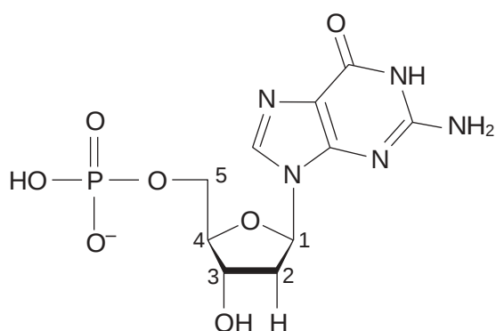
deoxyribonucleotide
