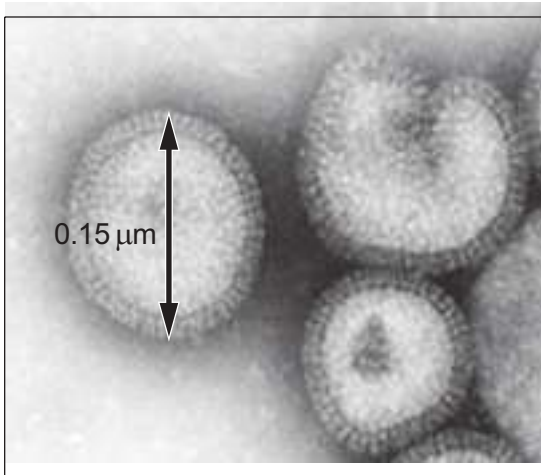
Flu virus Magnification = \times 200\,000
