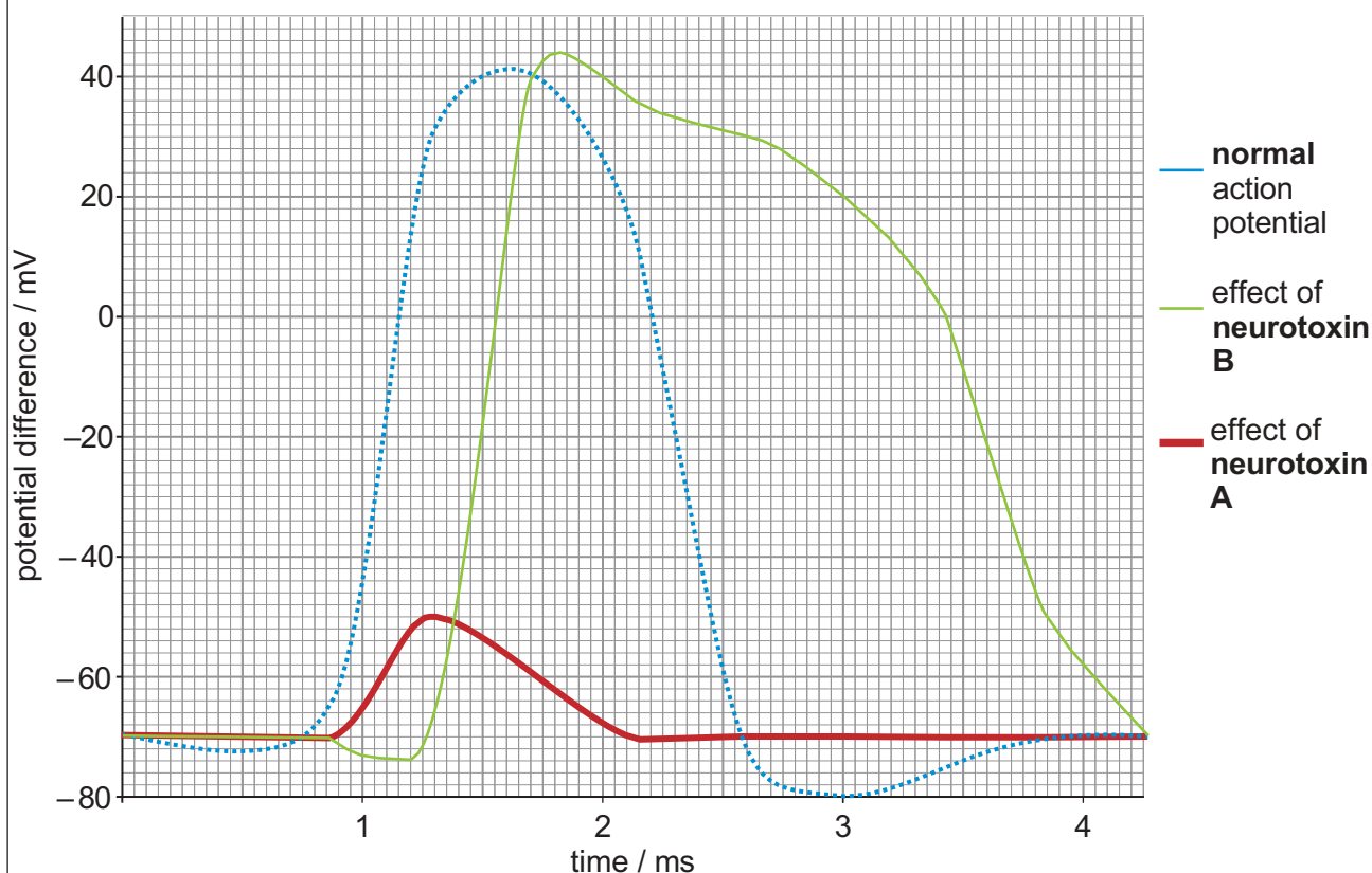
Effect of neurotoxins A and B on an action potential
