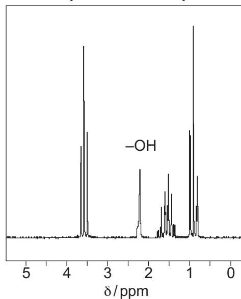
^1\text{H} NMR spectrum of compound A
