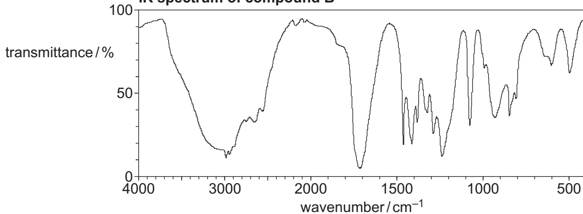
IR spectrum of compound B
