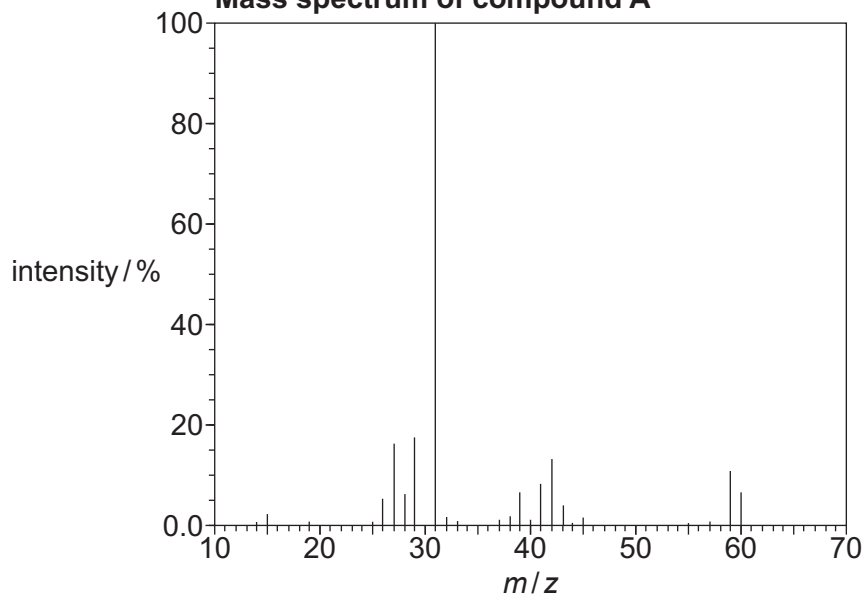
Mass spectrum of compound A
