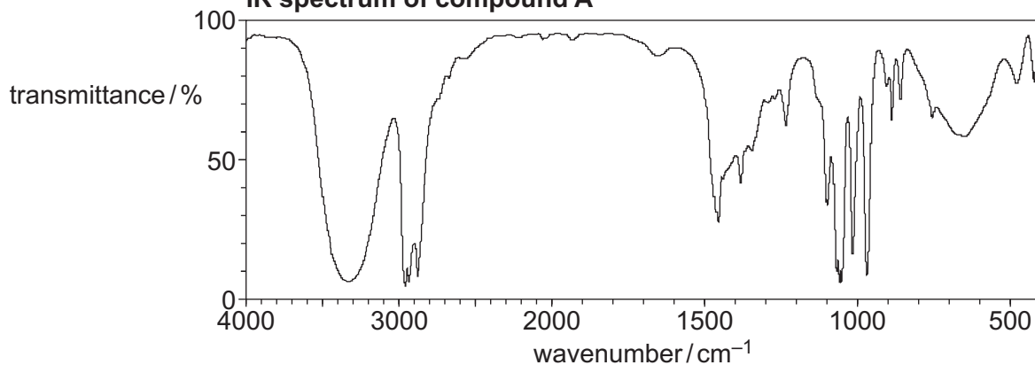
IR spectrum of compound A
